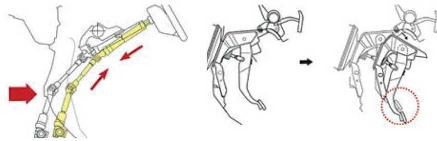
Collapsible steering shaft mechanism
