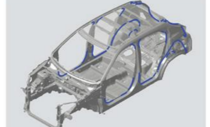
Structural adhesive bonding on doors and tailgate openings increases coupling rigidity between body parts. (Images are provided for illustrative purposes only.)
